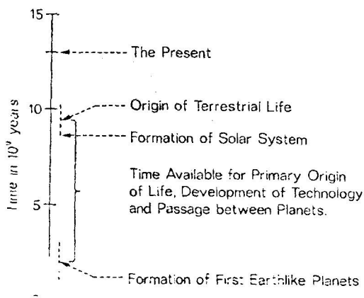
Figure 0 An approximate timescale for the Events discussed in this paper. To simplify the illustration, the age of the galaxy has been somewhat arbitrarily taken as 13 \times 10^9 years.
